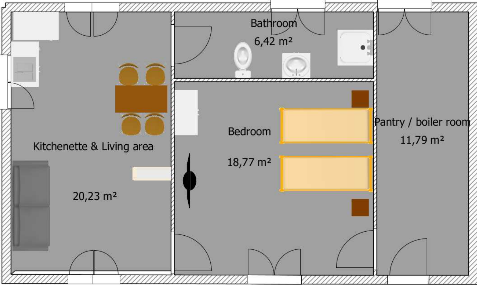
Guest house 10 x 6m
